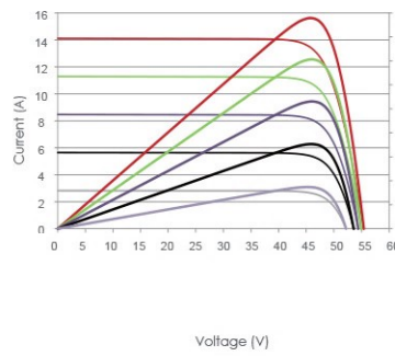
Current-Voltage & Power-Voltage Curves (615W)
